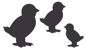
BABY CHICKENS
